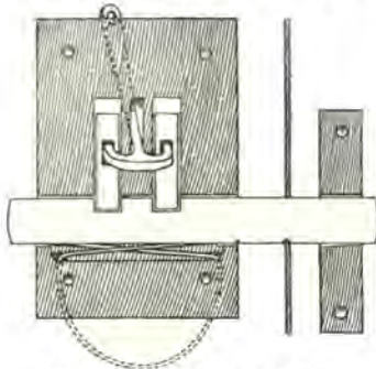
FIG. 184.—HOMERIC LOCK (RESTORED).
